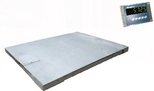
不锈钢秤体标配仪表AS131-SS AS131-SS Standard Configuration to Stainless Steel Scale body Indicator AS131-PL
