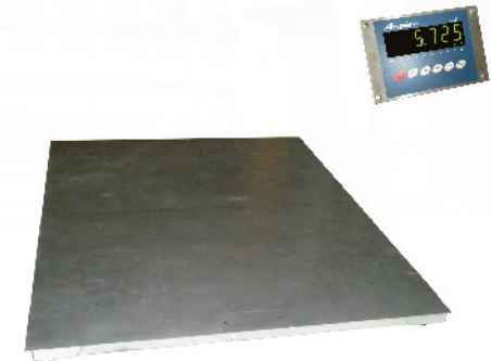
不锈钢秤体标配仪表AS131-SS Standard Configuration to Stainless Steel Scale body Indicator AS131-SS
