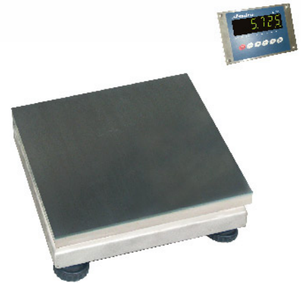
不锈钢秤体标配仪表AS131-SS Standard Configuration to Stainless Steel Scale body Indicator AS131-SS
